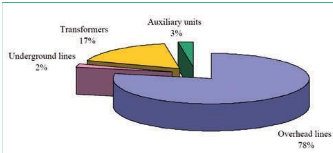
Example of breakdown of energy losses in the electricity transmission system
